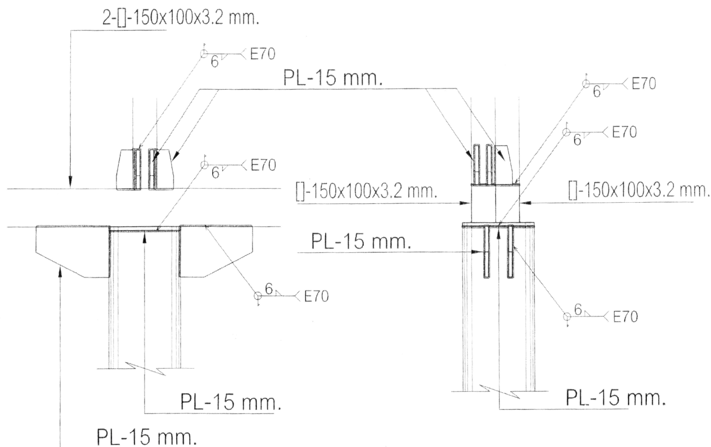
Column Detail 1:10
